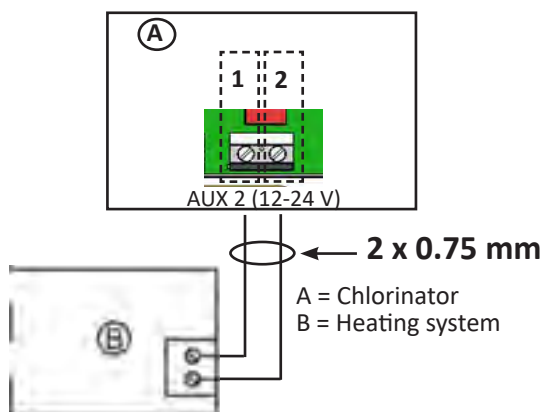
Connection of a heating system with remote on/off control
