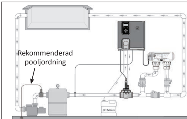
Installation i linje
